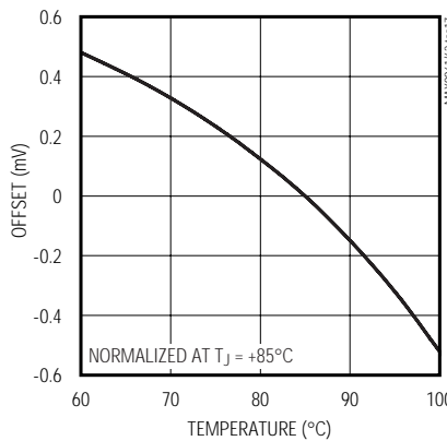
DRIVER OFFSET vs. TEMPERATURE
